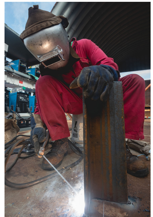
Wayne Jennings welds an angle bar to a deckplate. Photo by Matt Hildreth
