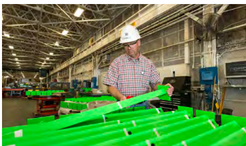
Shipbuilder Martin Conklin (O43) inspects the powder coating on tie-down stanchion posts. Photo by John Whalen
