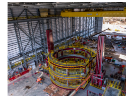
Cover Photo: NNS' first Advanced Fixture Assembly Machine in the Joint Manufacturing and Assembly Facility (JMAF) is scheduled to be fully operational in the fall. Photo by John Whalen
