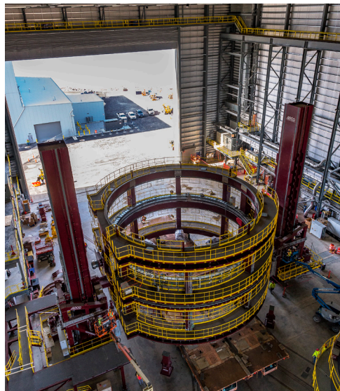
Shipbuilders and contractors work to connect the components of the Advanced Fixture Assembly Machine in the Fixture Production Bay. Photo by John Whalen
